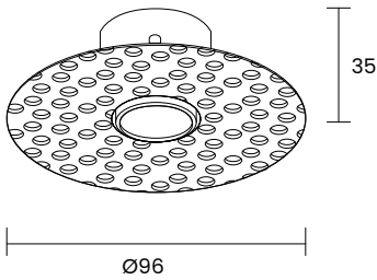
Code : CRZ06 Plasterboard flange for RAZE C6 W - White G - Grey B - Black
