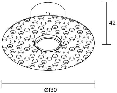
Code : CTR03 Plasterboard flange for MIRA 9 TRIMLESS MIRA 12 TRIMLESS
