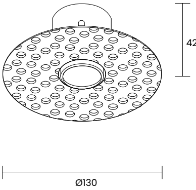
Code : CRZ08 Plasterboard flange for RAZE C12 W - White G - Grey B - Black
