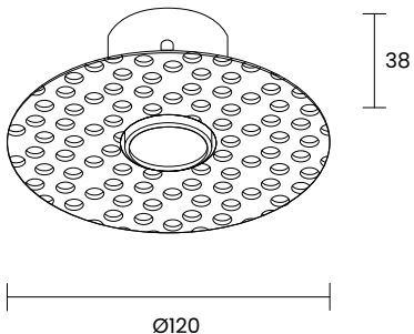
Code : CTR02 Plasterboard flange for PLUTONE TRIMLESS
