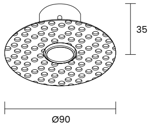
Code : CRZ03 Plasterboard flange for RAZE 6 W - White G - Grey B - Black
