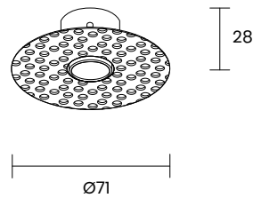
Code : CRZ19 Plasterboard flange for PHANTOM, PHANTOM PLUS W - White G - Grey B - Black
