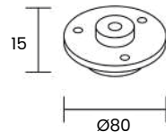
Code : BAS01 Base for one unit for: JUNCUS
