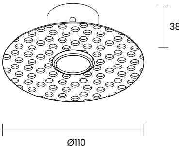
Code : CTR01 Plasterboard flange for VENUS TRIMLESS
