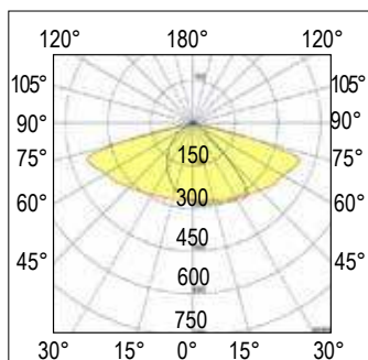
ST/CDL3 Ottica stradale consigliata per piste ciclabili Street optic recommended for cycle paths
