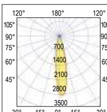
15° Super spot
