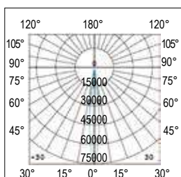
15° Semi-concentrante Spot
