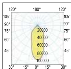
35° Concentrante - Concentrating
