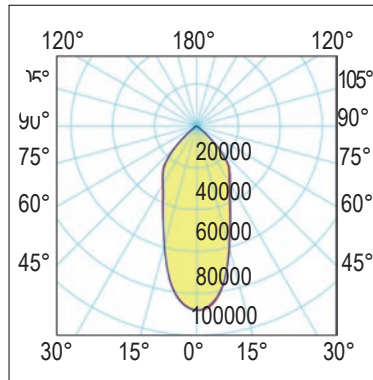
35° Concentrate - Concentrating
