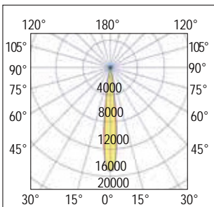
15° - Super spot
