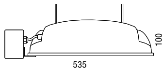
LED Zeus + Sensor Dimensioni (mm) - Dimensions (mm)
