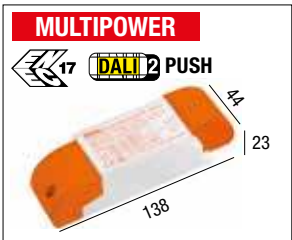
LED driver multipower RN8166 DALI 2 PUSH (DALI, PUSH, 0-10V.)
