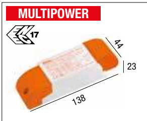
LED driver multipower RN8167 (ON-OFF)
