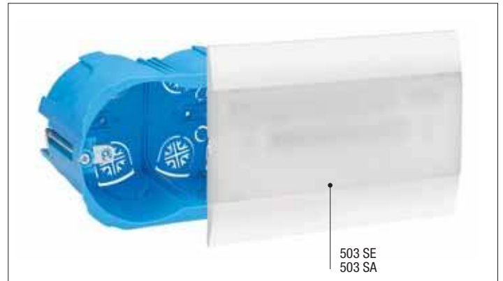
Incasso cartongesso Recessed plasterboard
