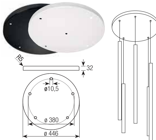
ROSONE TONDO Ø 445 - 5 FORI ROUND CEILING ROSE Ø 445 - 5 HOLES
