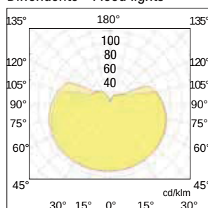
Diffondente - Flood lights
